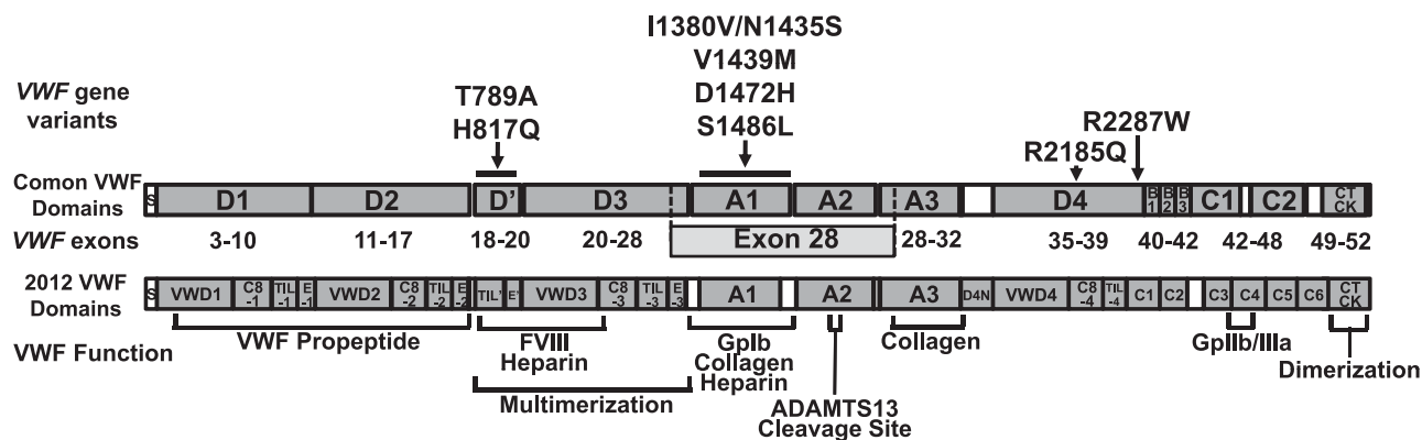
Figure 1. Scale schematic of VWF missense variants associated with levels of VWF or FVIII levels in African Americans (AAs). The location of each of VWF variants with significant univariate associations with VWF and/or FVIII levels in AAs are indicated by arrows to the corresponding commonly annotated VWF domain (top). An alignment with the recently revised VWF domain annotation 6 is also shown (bottom). Two variants, I1380V and N1435S, are in strong LD ( r^2 = 0.89 ) and are therefore represented together.
